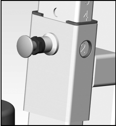
Figure 11: Lubricate the snap pin by pulling it out
