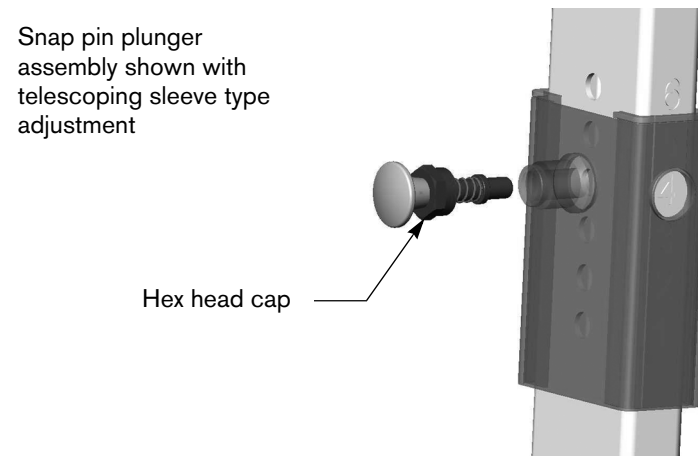
Figure 12: Inspect snap pins (snap pin shown in exploded view for clarity)
